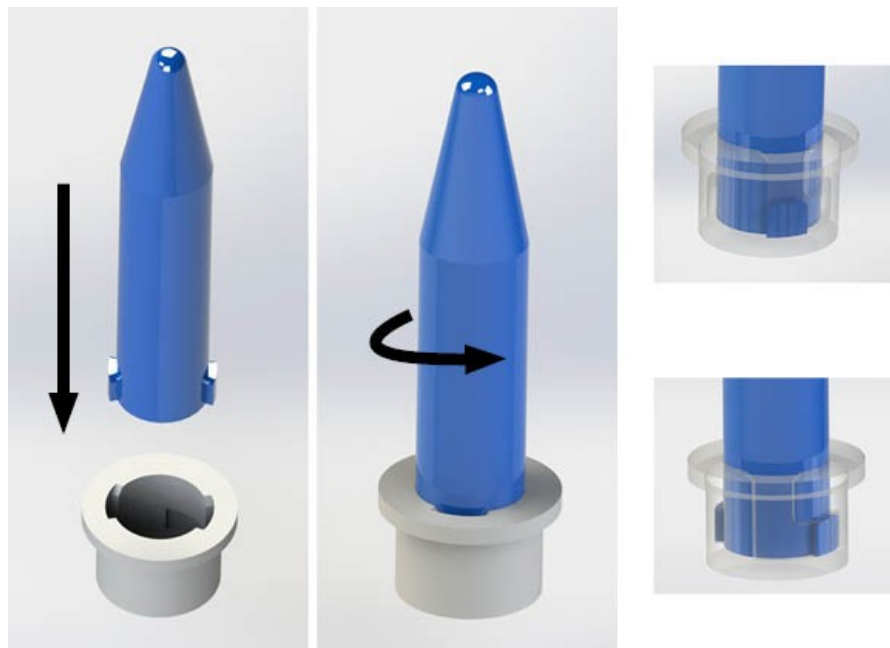
Figure 21: Penholder mechanism
